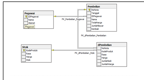
Gambar 3.8 Relasi Antar Tabel Database.
