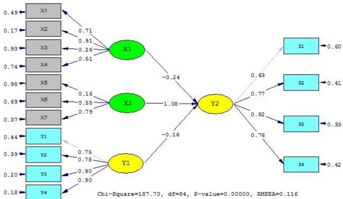
Gambar 3 - The Path Coefficient Sub-Structure 2
