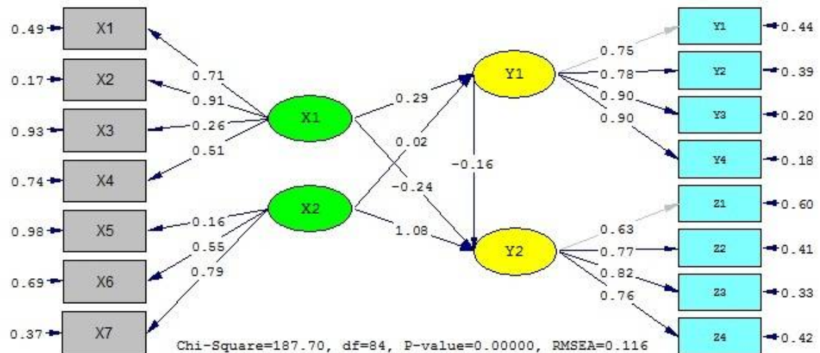
Gambar 4. - The Path Coefficient Sub-Structure 2
