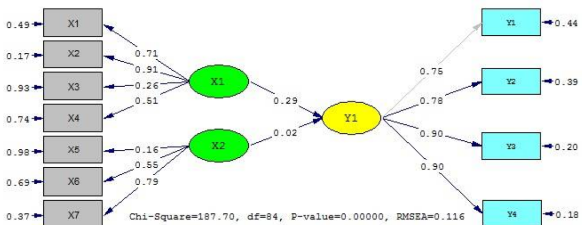
Gambar 2 - The Path Coefficient Sub-Structure 1
