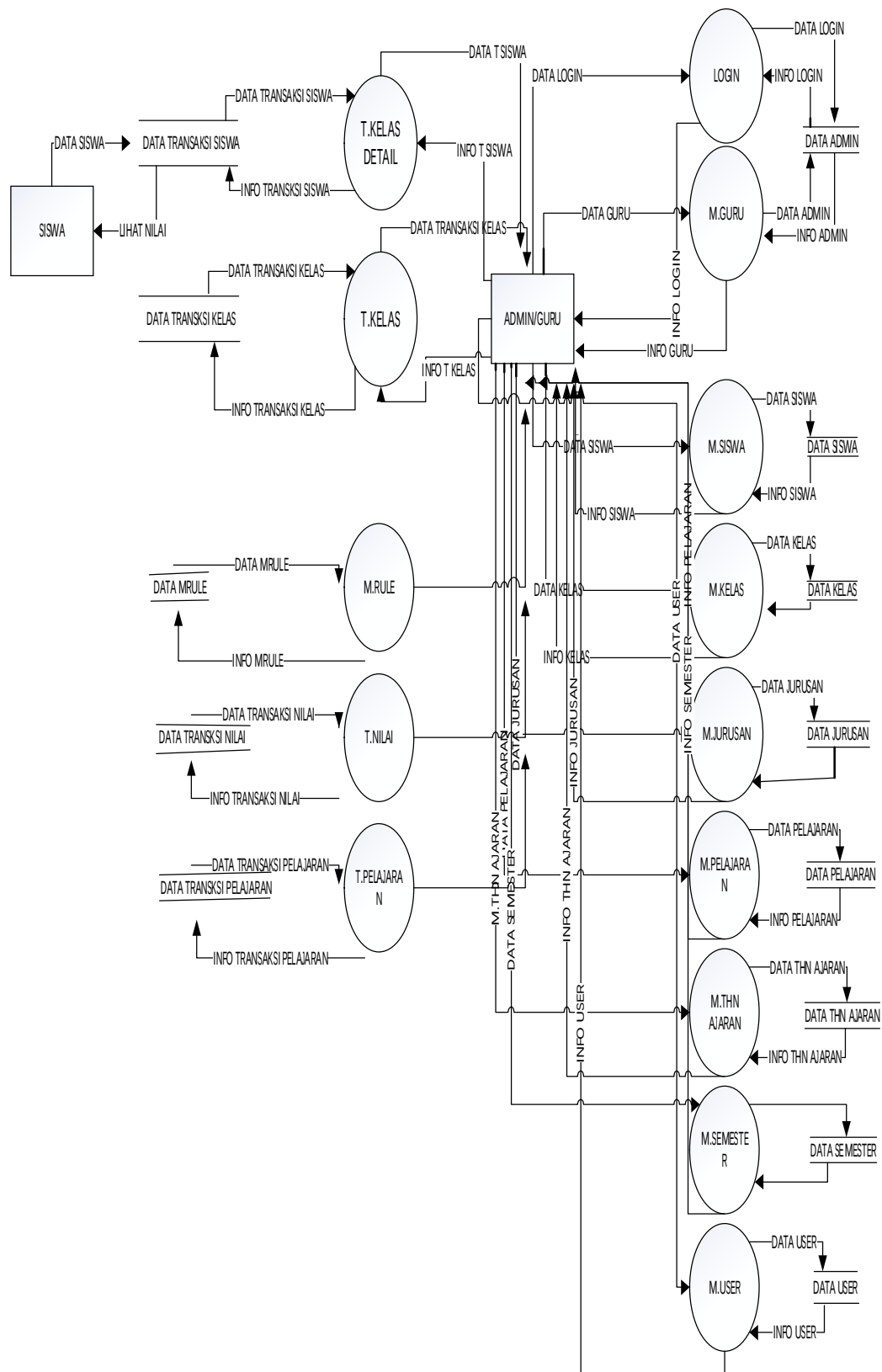
Gambar2.2Context Diagram
