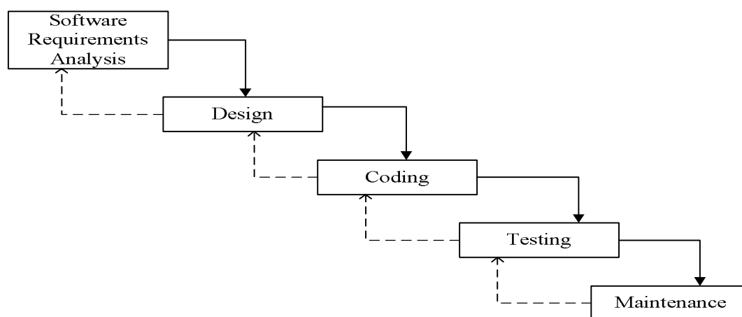
Gambar 2.1Metode Waterfall(Mall, 2003)
