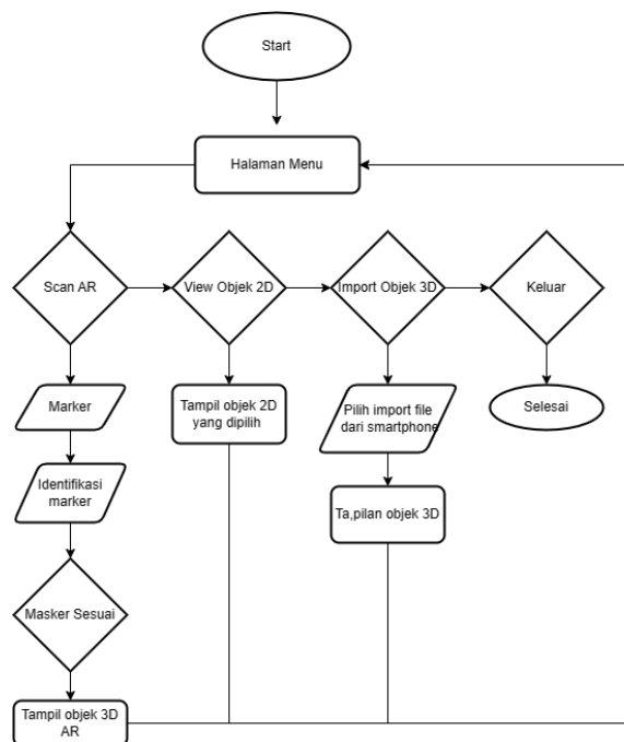
Gambar 2. Flowchart Diagram
