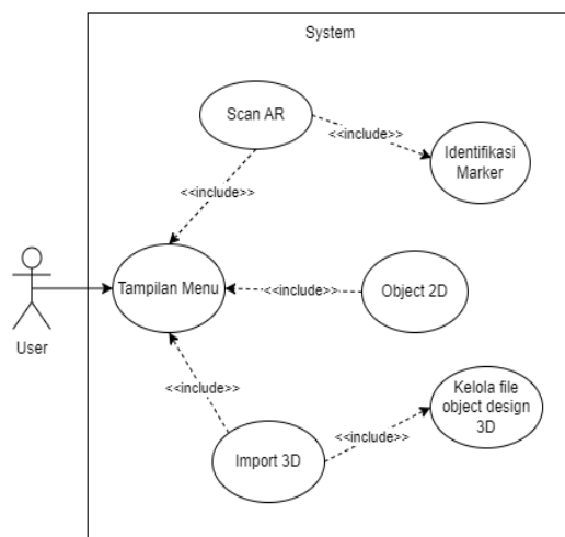
Gambar 3. Usecase Diagram
