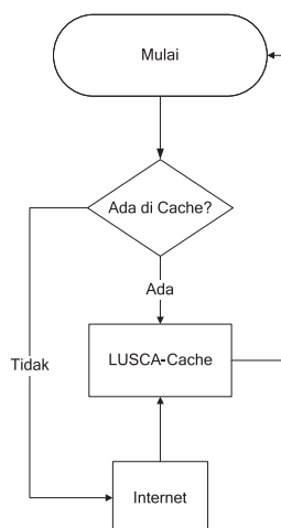
Gambar 2. Flowchart LUSCA-Cache
